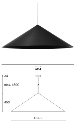
w151 Extra large pendant s3
