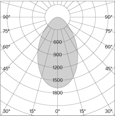
w151 Extra large pendant s1 3000 K / traffic white
