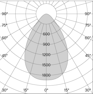
w151 Extra large pendant s2 3000 K / traffic white
