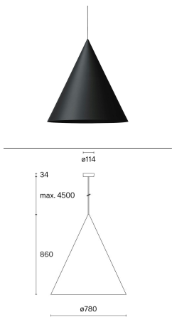
w151 Extra large pendant s2
